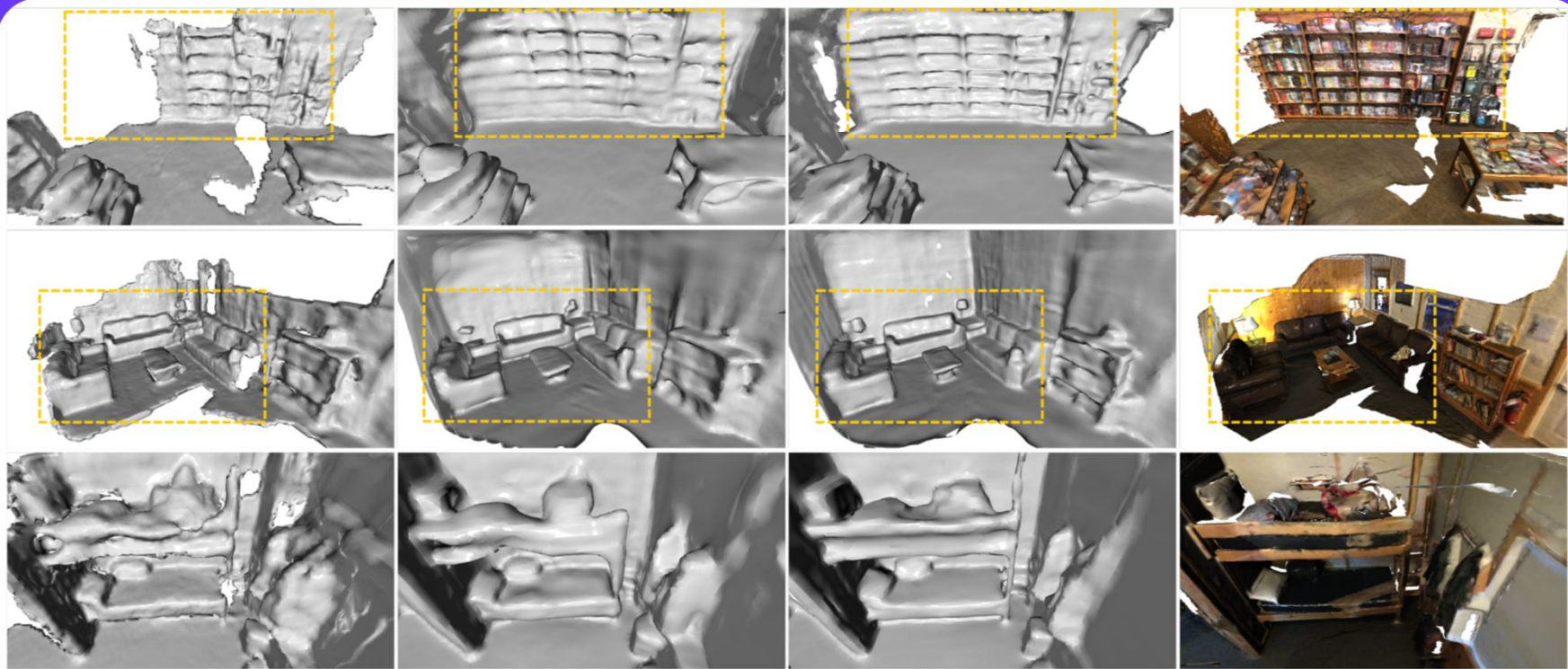
NeuralRecon
